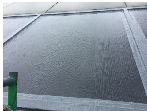
Sikalastic® Clearglaze is applied by foam roller at 20 mils WFT (80ft 2 /gal) per coat. Lap up onto the installed RoofPro membrane 2 inches butting up against the mullion.
