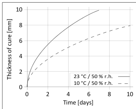
Diagram 1: Curing speed for Sikaflex®-292
