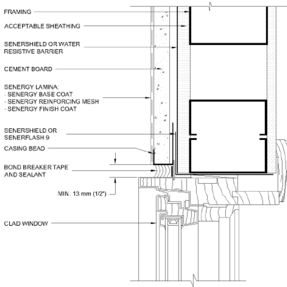
FIGURE 5—TYPICAL CLAD WINDOW JAMB DETAIL
