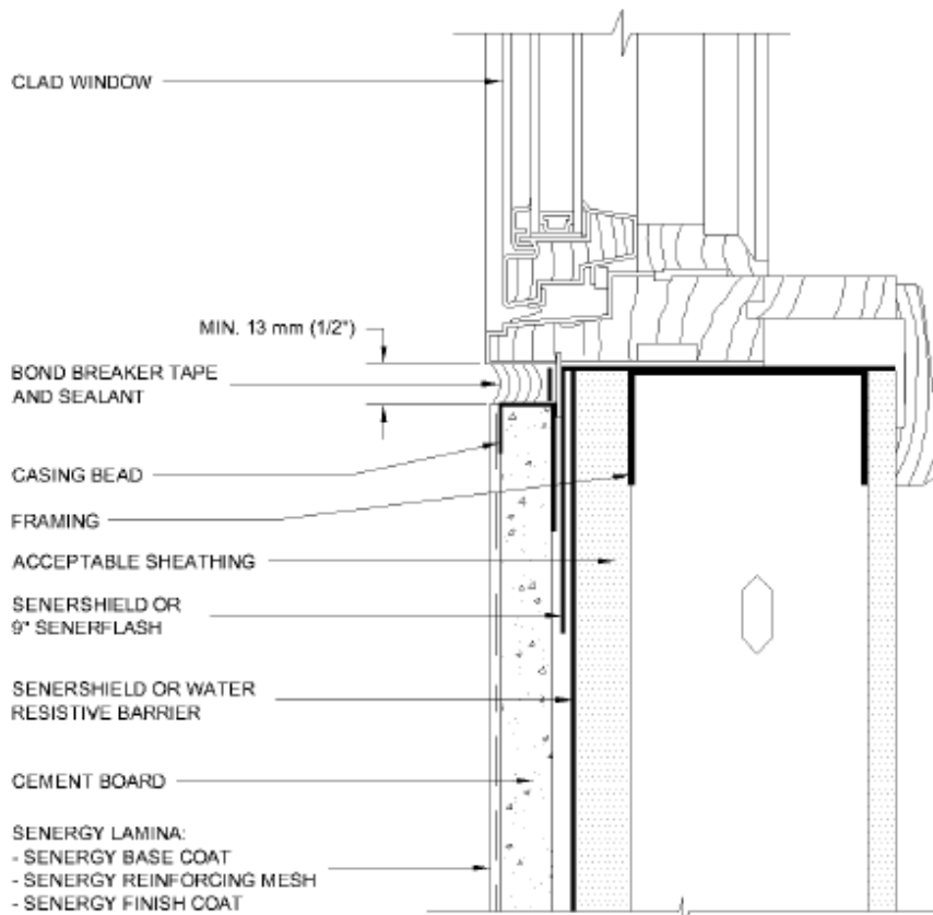
FIGURE 6—TYPICAL CLAD WINDOW SILL DETAIL
