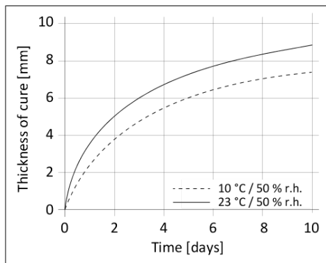
Diagram 1: Curing speed for Sikaflex®-292i
