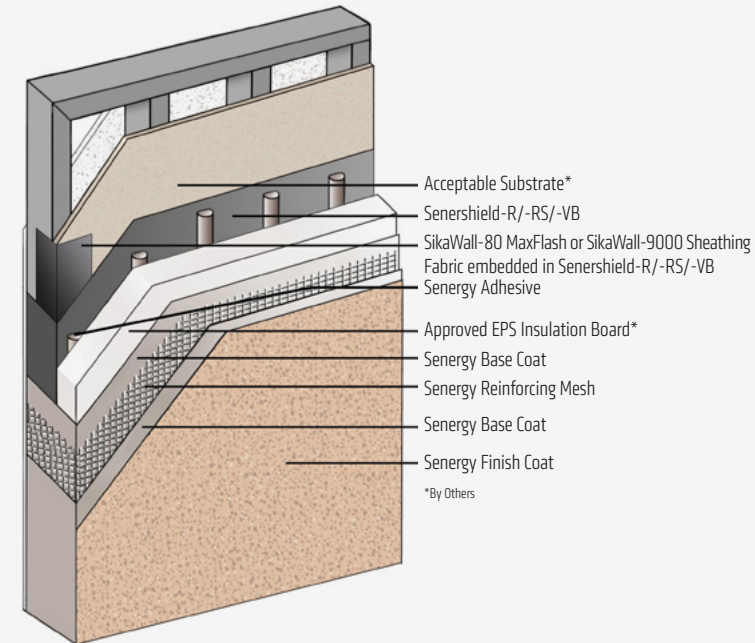
SenerPanel Secondary Weather Barrier
