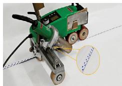
Thermochromic Welding Indicator
