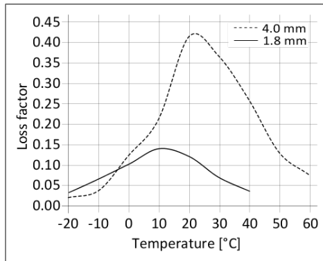
Diagram 1: Loss factor SikaDamp®-111 at 200 Hz
