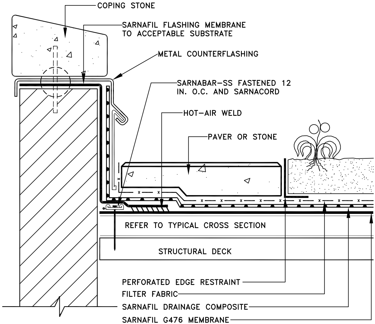
ATL. BASE DETAIL
