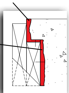
2 1/2" Cantilevered Cut Stone Step Liner
