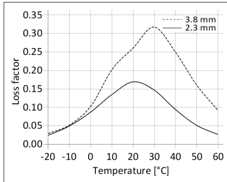
Diagram 1: Loss factor SikaDamp®-112 PP at 200 Hz
