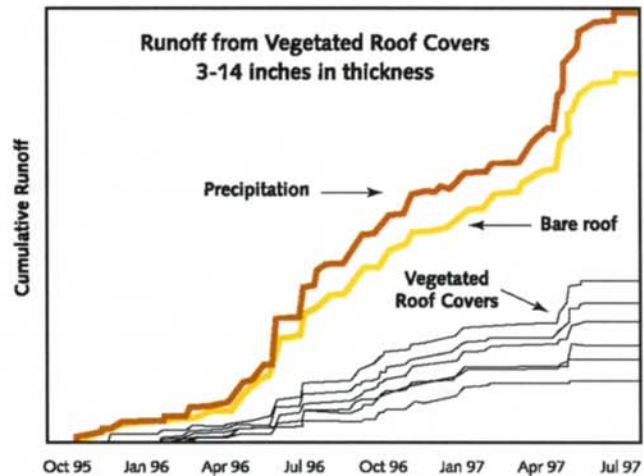
Chart 1: Stormwater Reduction Chart, courtesy of Roofscapes Inc., Philadelphia, PA.
