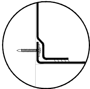
SARNASTOP AT BASE OF WALL OR CURB ALTERNATE BASE FASTENING
