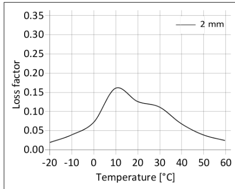
Diagram 1: loss factor SikaDamp®-110 PP at 200 Hz
