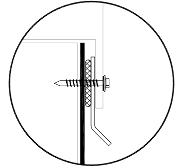
SIKAFLEX-1A APPLIED UNDER METAL EXTENDER PIECE
