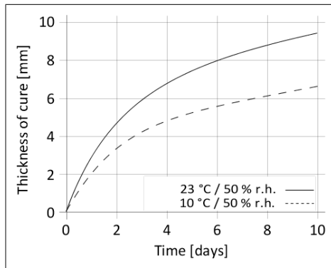
Diagram 1: Curing speed Sikaflex®-505 UV Hi Visc
