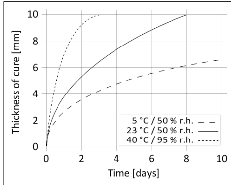
Diagram 1: Curing speed Sikasil® WS-605 S
