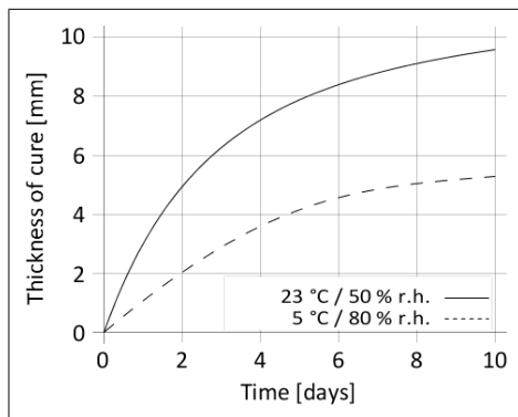
Diagram 1: Curing speed Sikaflex®-250 UF-1P
